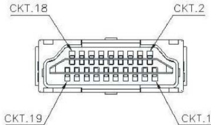
HDMI Type A Connector Pin Assignment
